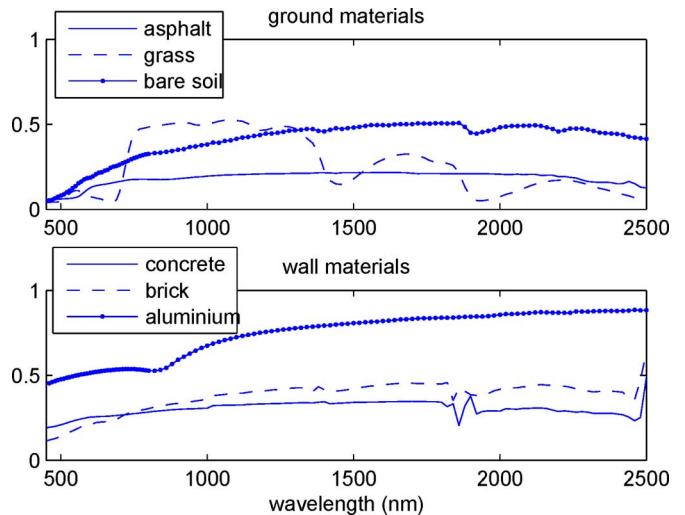
Fig. 1. Reflectance spectra of used materials.
