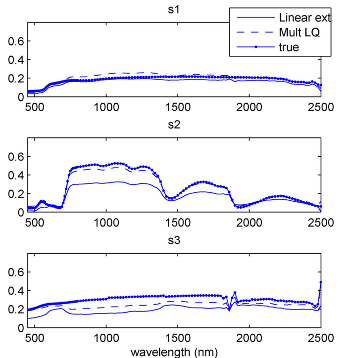
Fig. 2. Example of estimated spectra with Linear ext ( SAM = 0.12 ) and Mult LQ ( SAM = 0.09 ).
